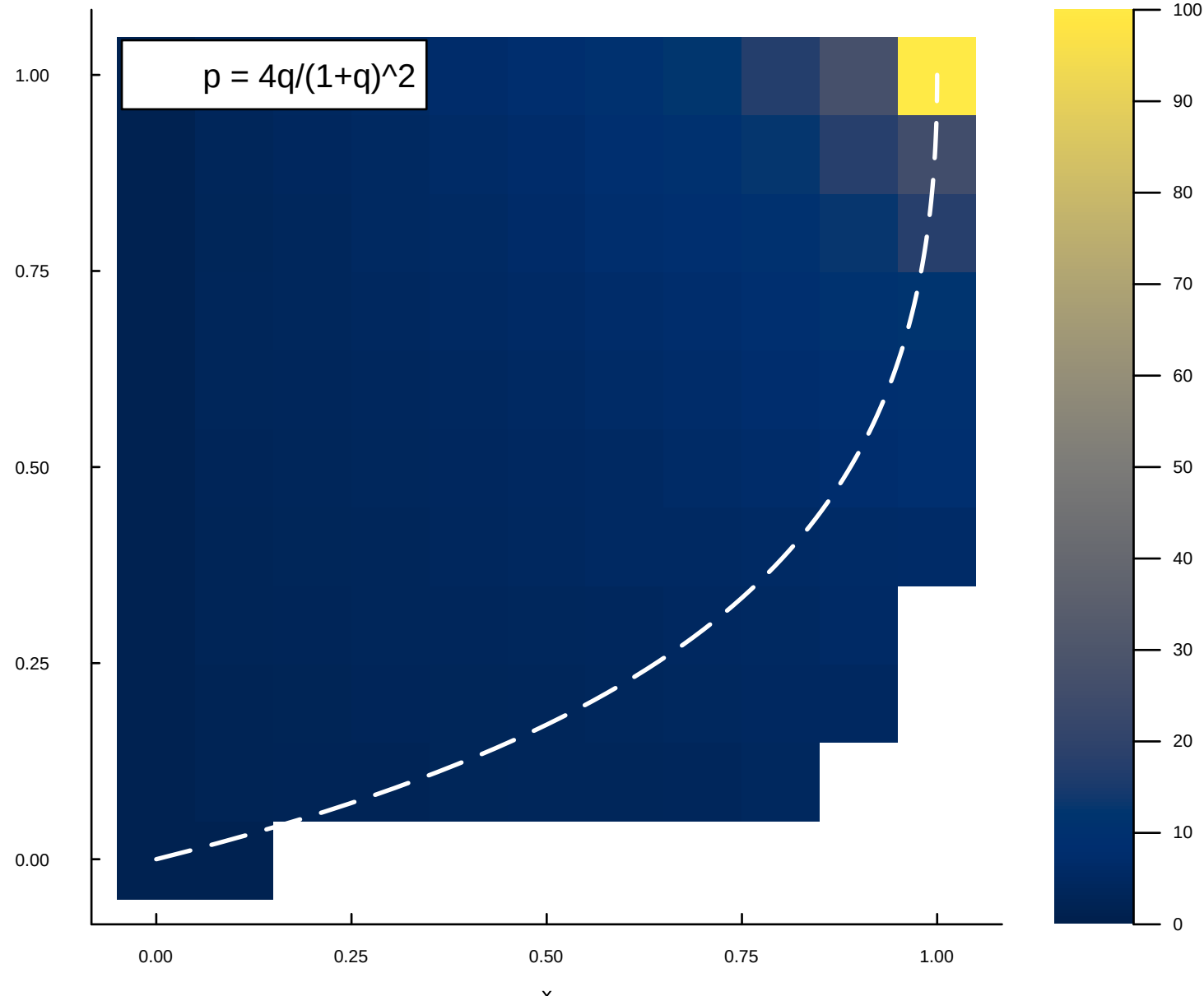
Fixed Point Realizations
